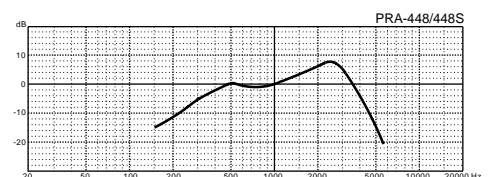
Frequency Response
