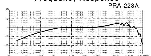
Frequency Response
