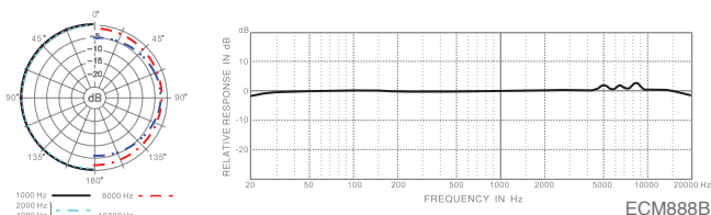
ECM888B Frequency Response (Omni)
