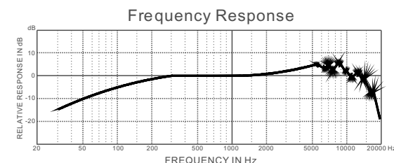
Tom tom 典型频率响应 (图4)
