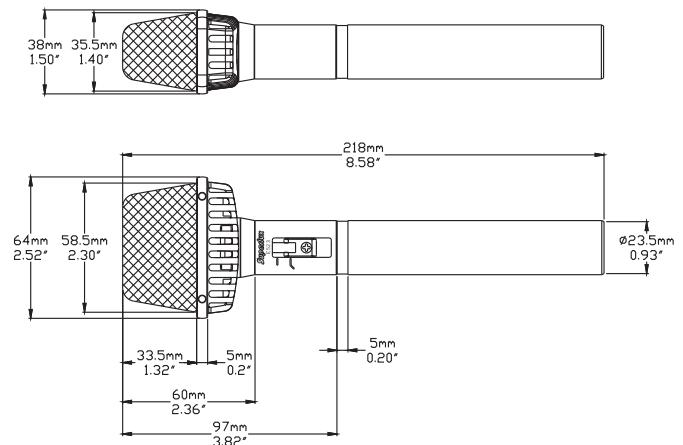
Figure of Exterior Dimensions
