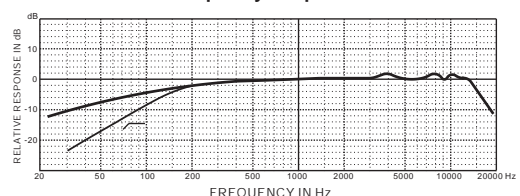
Frequency Response
