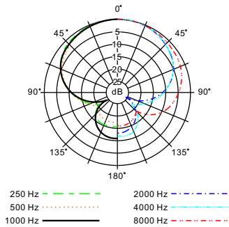
Polar Pattern
