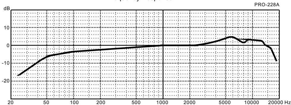
Frequency Response
